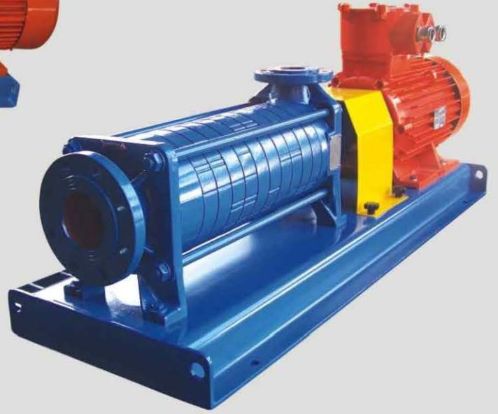
Model No: LPG 250-5 / Kapasite 25 m 3 /h 20 Bar Model No: LPG 250-5 / Capacity 25 m 3 /h 20 Bar
